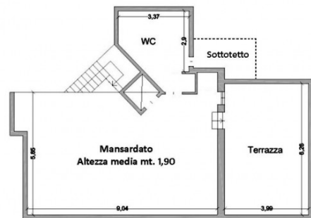
PIANO MANSARDATO
